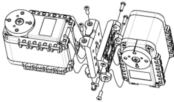
Exploded view
