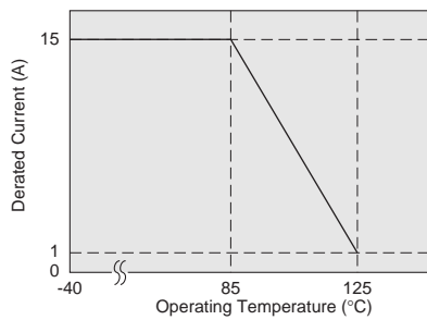
Derating
